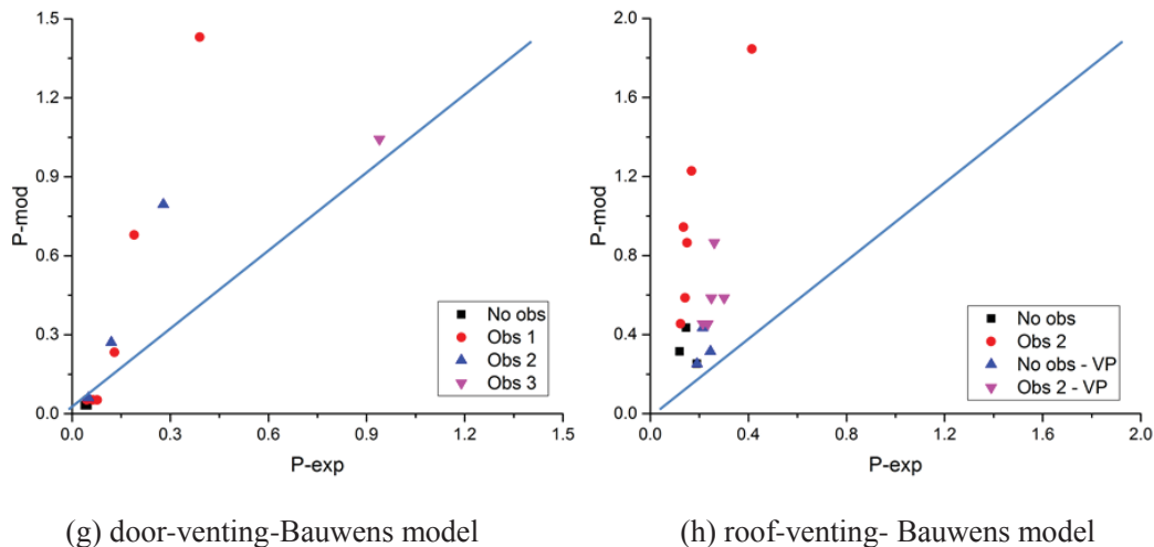
Figure 7. Comparison of the measured and calculated values of overpressure for 20 feet ISO container data for cases having door-venting and roof-venting using EN-14994 (a-b), NFPA, (c-d) Molkov and Bragin model (e-f), Bauwens et al. model (g-h). Some cases with vent panel are also discussed (VP)
